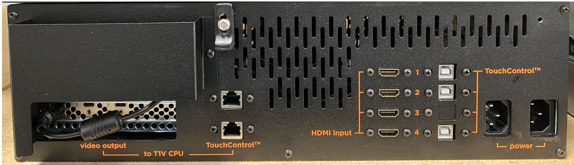
Rear panel
